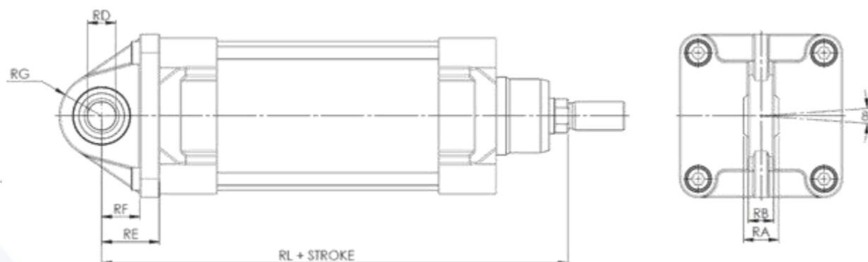
Male hinge with ball joint (MP6), Material aluminium RA or steel RS Example. RA 050 20 STD
