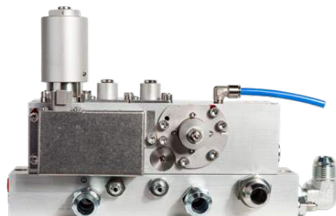
Valve blocks
