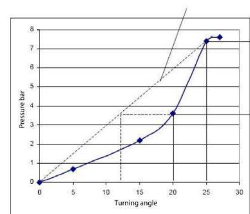
Servo valves that are generally available on the market
