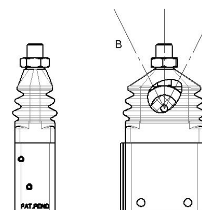
Locking positions A and B
