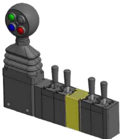
SUPPLY MODULE MIDDLE. INLET AND EXHAUST PORTS ON THE BOTTOM Type 9130-MSP-030557
